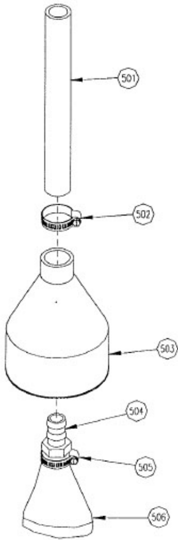
BOOT DROP ASSEMBLY
