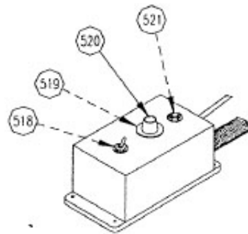
CAB CONTROL ASSEMBLY P/N: RHAB371
